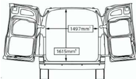
SLWB Panel Van with barn-door style tailgate
