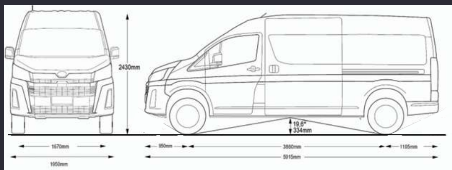
Quantum / HiAce 4x4 Dimensions - Super Long Wheel Base / High Roof
