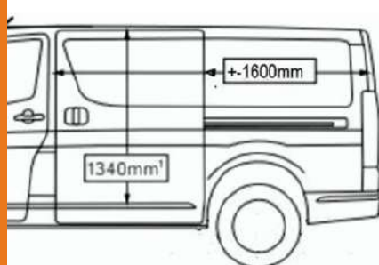
LWB Crew Cab
